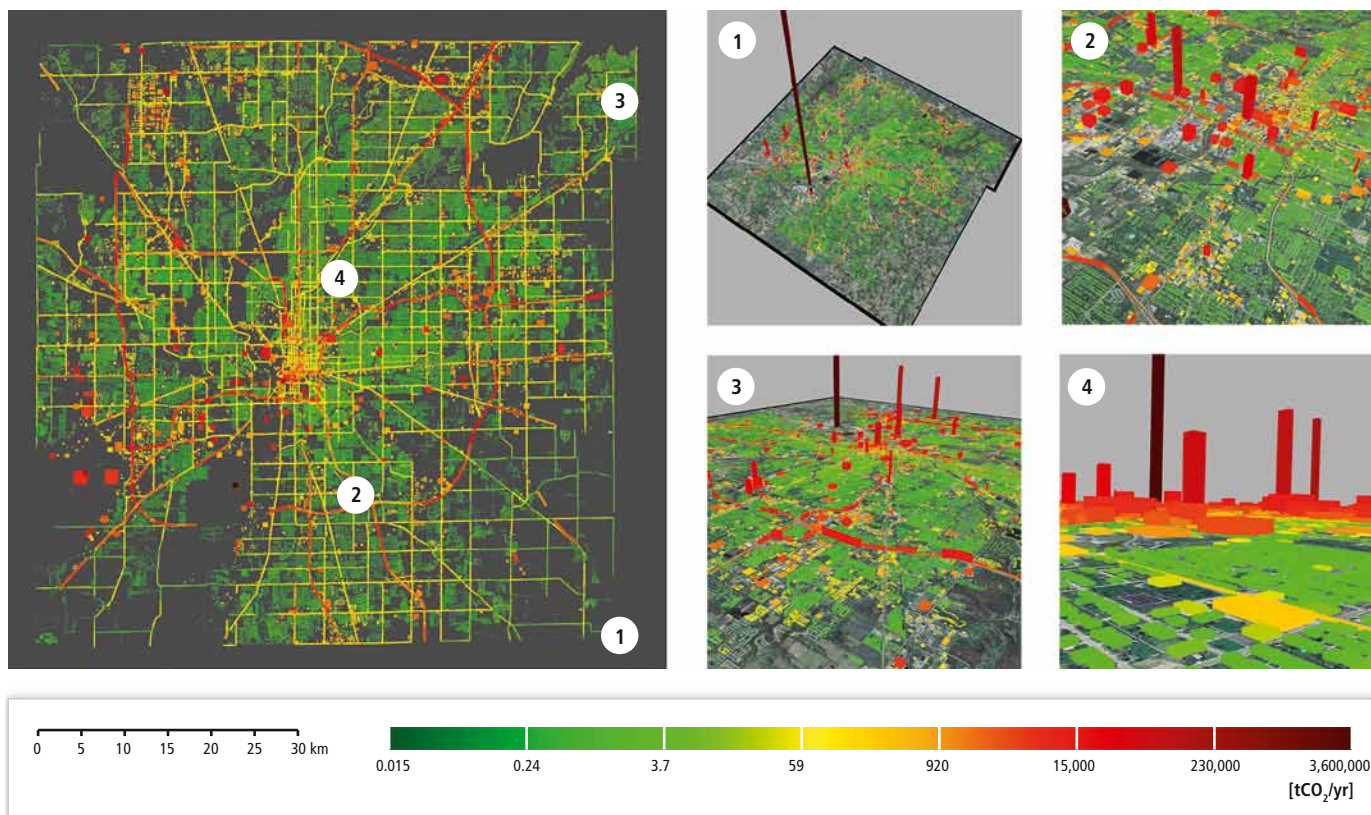
Figure 12.7 | Total fossil fuel emissions of Marion County, Indiana, USA, for the year 2002. Left map: Top-down view with numbered zones. Right four panels: Blow ups of numbered zones. Box height units: Linear. Source: Gurney et al. (2012).
