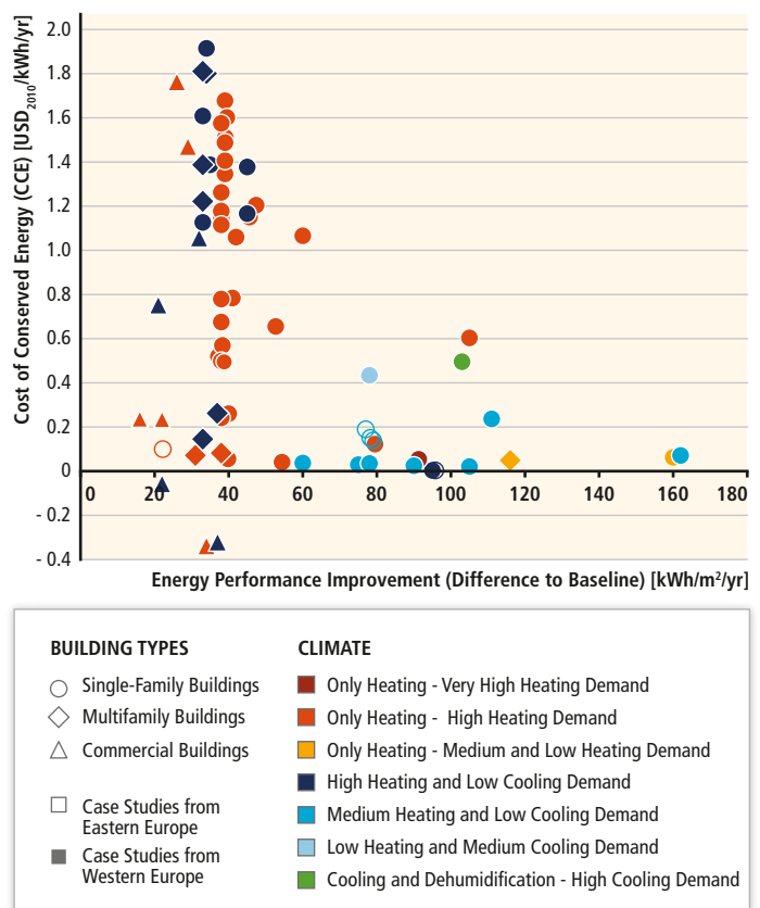
Figure 9.14 | Cost of conserved energy as a function of energy performance improvement ( \text{kWh}/\text{m}^2/\text{yr} difference to baseline) to reach ‘Passive House’ or more stringent performance levels, for new construction by different building types and climate zones in Europe. A discount rate of 3 % and the lifetime of 30 years for retrofit and 40 years for new buildings have been assumed. Sources: Hermelink (2006), Galvin (2010), ETK (2011), Gardiner and Theobald (2011), Nieminen (2011), Energy Institute Vorarlberg (2013), PHI (2013), Harvey (2013).
