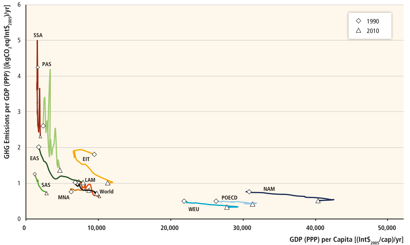
Figure 14.6 | Relationship between GHG emissions per capita and GDP per capita (top panel), and GHG emissions per GDP and GDP and per capita (bottom panel) (1990–2010). Data sources: GHG emission data (in CO 2 eq using 100-year GWP values) from JRC/PBL (2013) and IEA (2012a), see Annex II.9; GDP (PPP) from World Bank (2013a); and population data from United Nations (2013).
