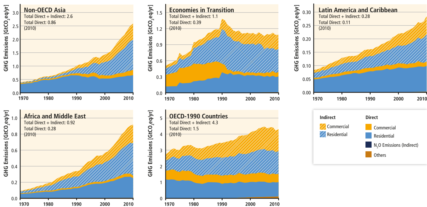
Figure 9.2 | Regional direct and indirect emissions in the building subsectors (IEA, 2012a; JRC/PBL, 2013; see Annex II.9).
